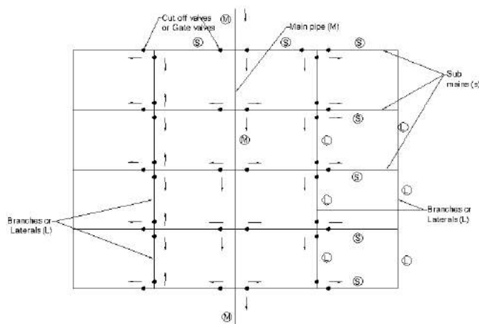
Figure 2.3: Grid-iron system
